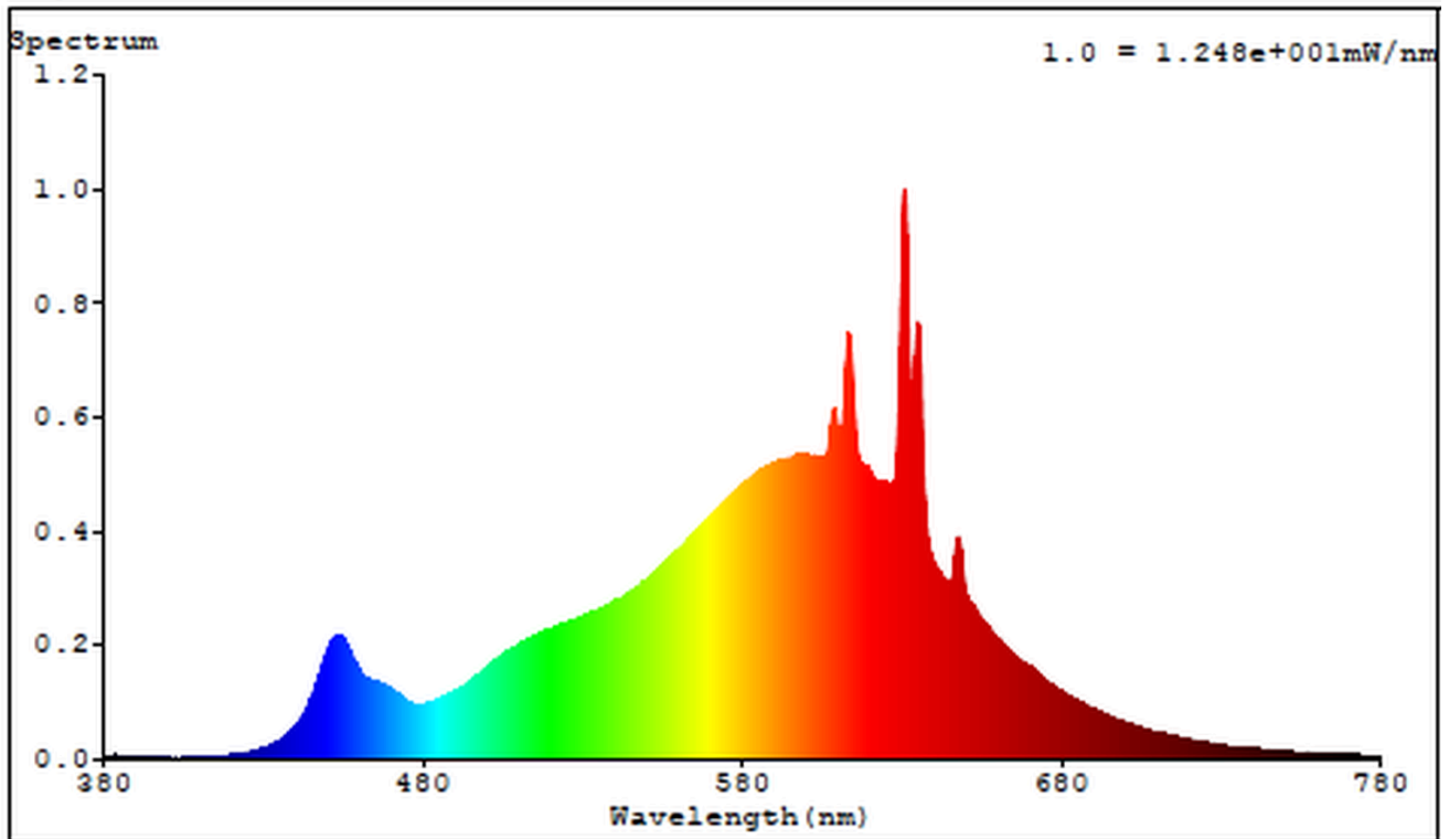
Spectral Distribution
